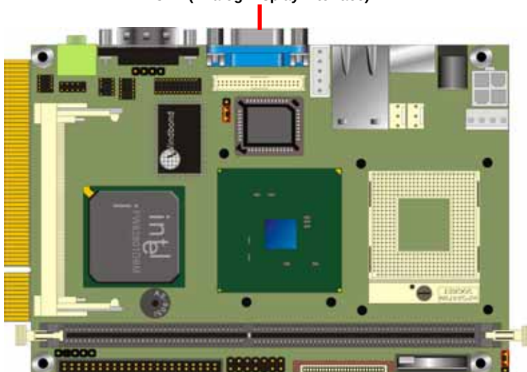
CRT (Analog Display Interface)
