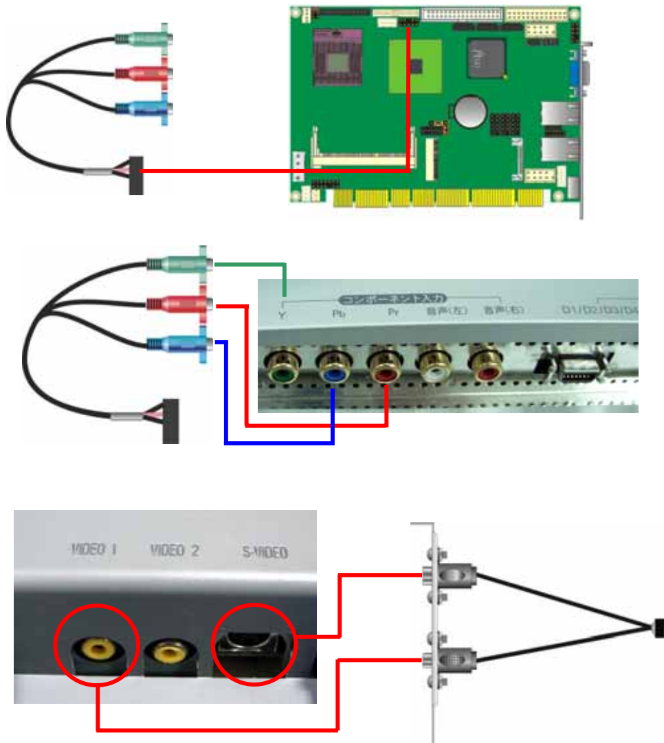
YPrPb Component Cable (For HDTV)
